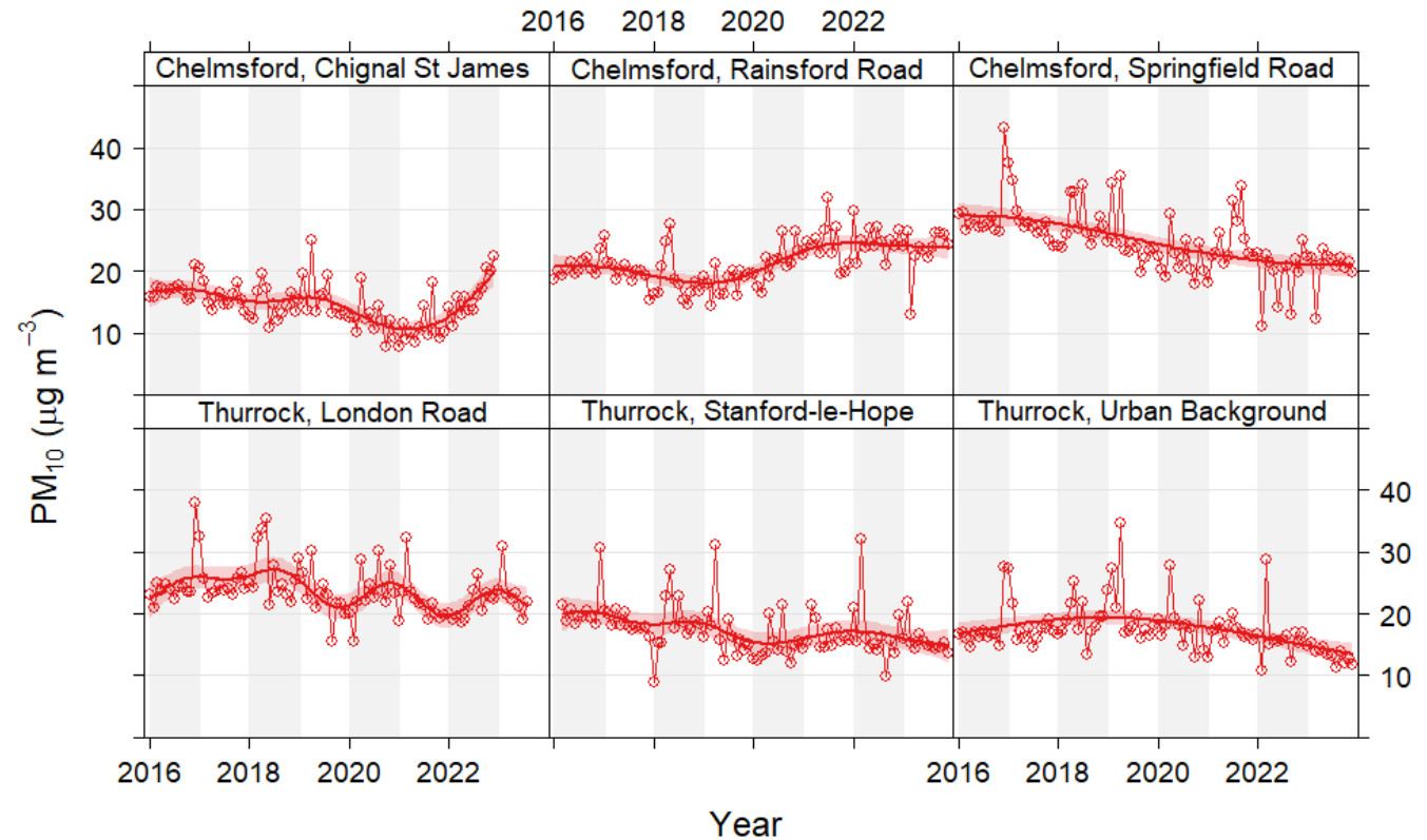
Figure 13 Observed trends in PM 10 concentrations at monitoring sites in Essex
